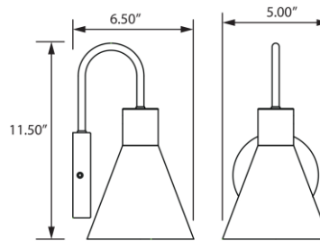
LINE DRAWING
