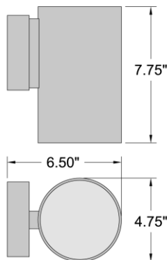
LINE DRAWING
