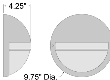
LINE DRAWING
