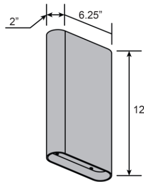
LINE DRAWING
