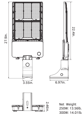
250W / 300W (Pole Mount)
